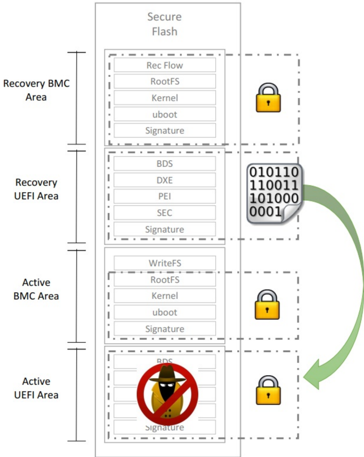
Figure 4-5: Cerberus recovery flow (source: “Project Cerberus Hardware Security”)
